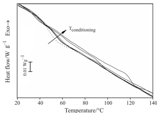
Fig. 1 DSC traces for PBT cubic specimens rapidly cooled in liquid nitrogen from room temperature (dotted line) and from higher conditioning temperatures (solid line; T_{\text{COND}}=35, 45, 60, 80 and 100^\circ\text{C} )
