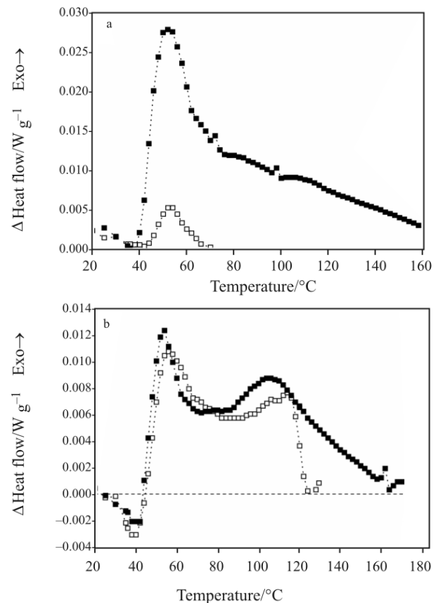
Fig. 3 Differential heat flow, \Delta(\text{Heat flow}) , measured in DSC tests on \blacksquare – specimens deformed at \epsilon_0=30\% and \square – undeformed specimens for corresponding values of conditioning and deformation temperatures, after quenching in liquid nitrogen: a – T_{\text{COND}}=T_{\text{DEF}}=45^\circ\text{C} and b – T_{\text{COND}}=T_{\text{DEF}}=100^\circ\text{C}
